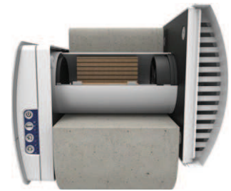
With mounting frame for thin walls
